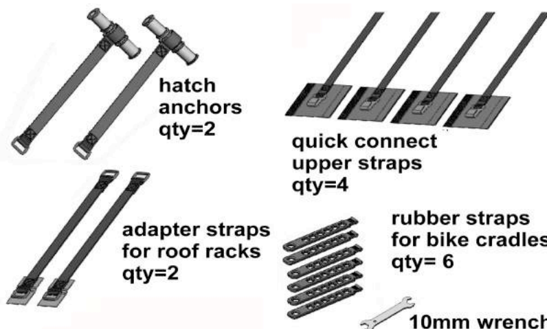
Fig. 2: Parts included with F2 Rack
